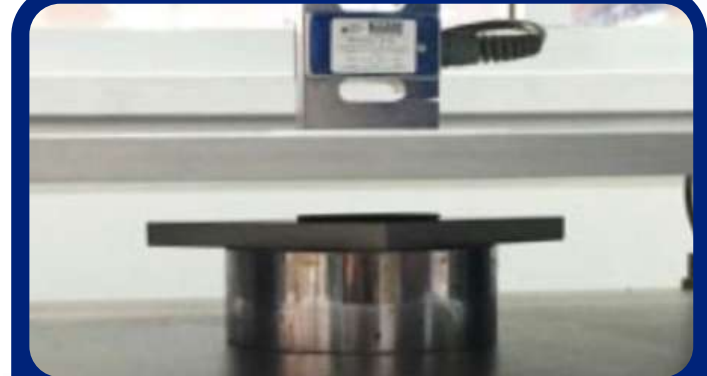
Flat Crush Resistance (FCT)
